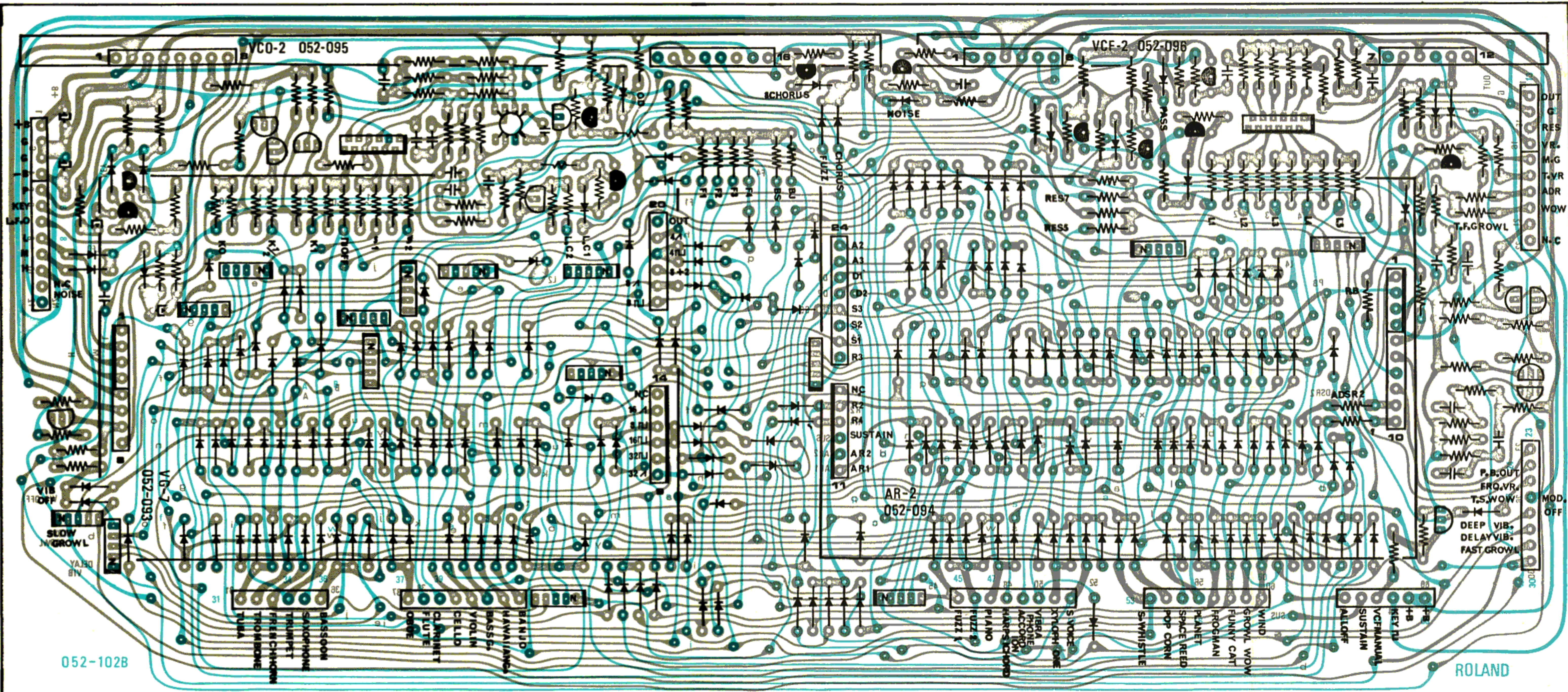
9-5. Both Side Circuit Patterns of MX-1 Board
